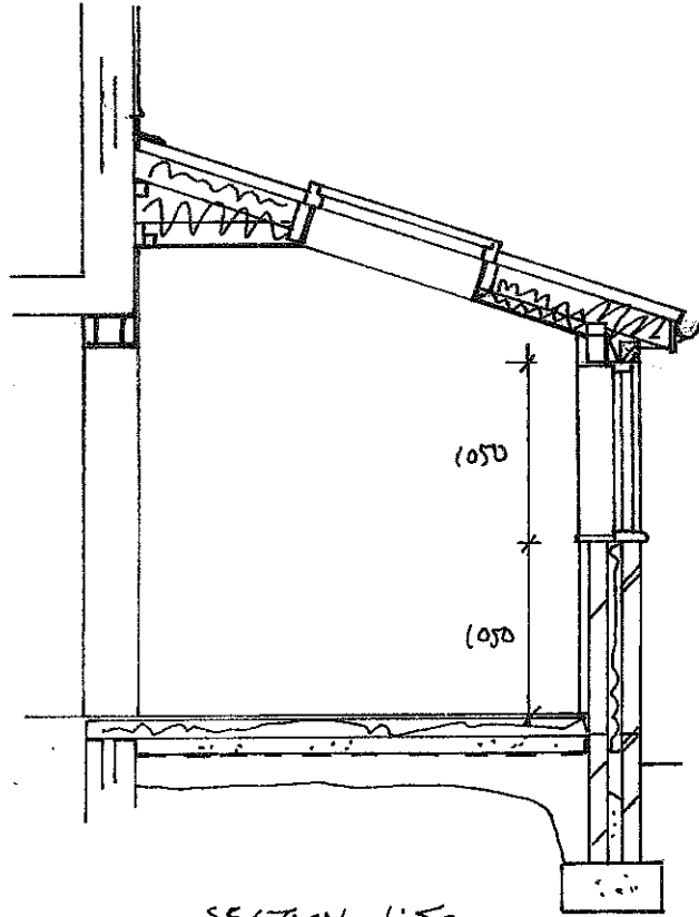
SECTION 1:50
